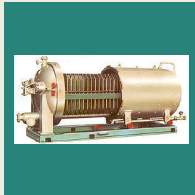
Horizontal Leaf Filter
