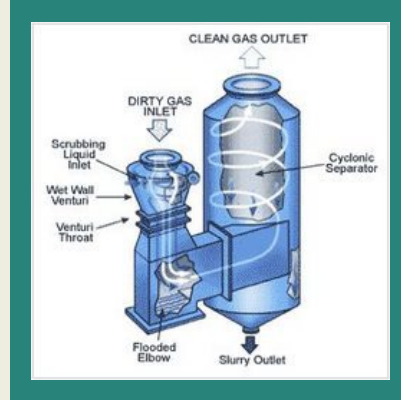
Wet Scrubbers
